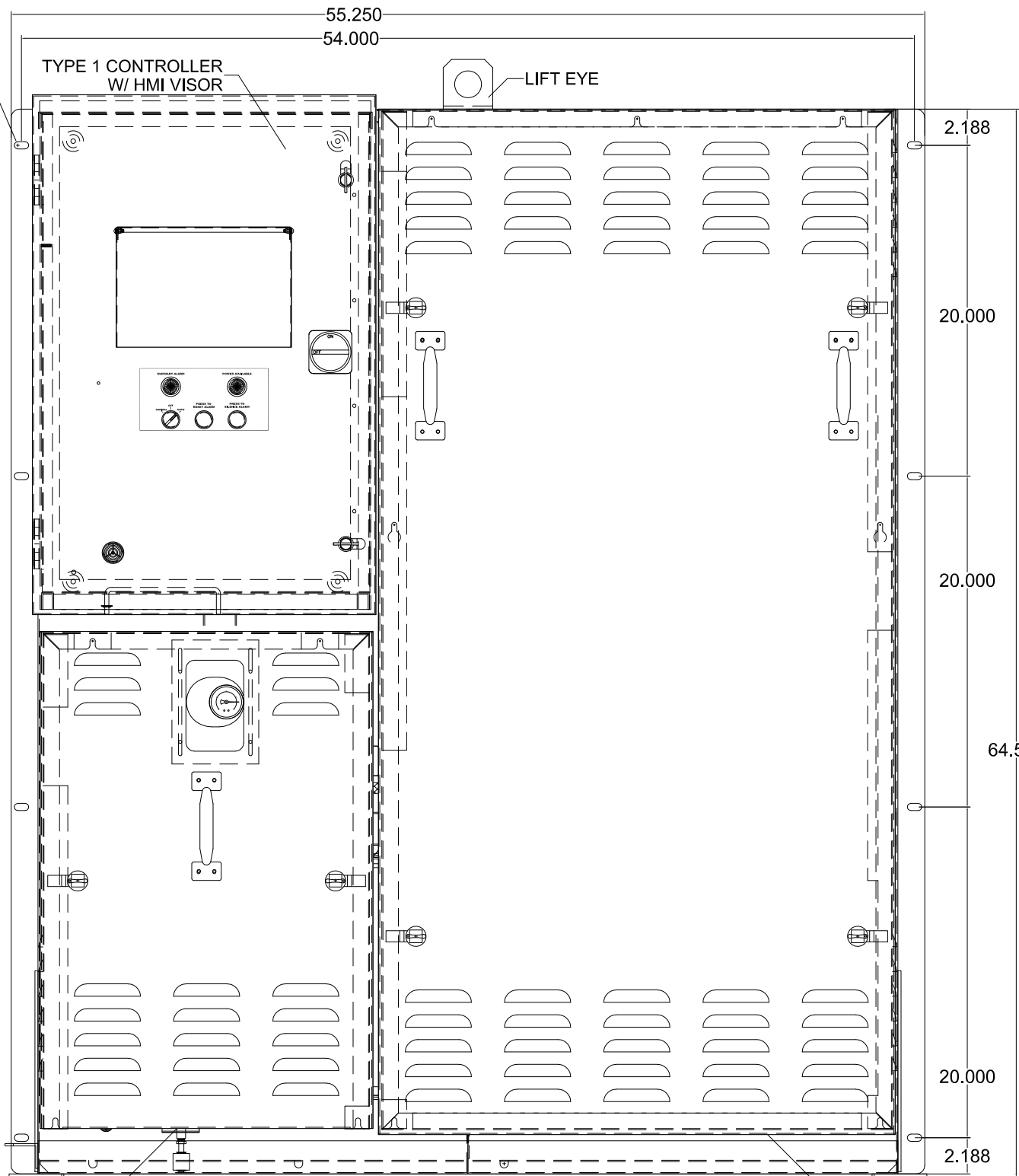
FRONT VIEW
