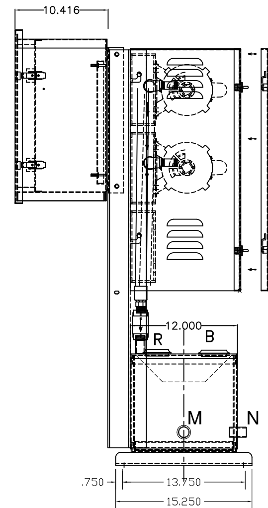
RIGHT VIEW
