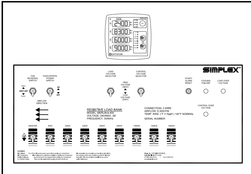
Part of Typical Merlin 400 Local Control Detail Drawing
